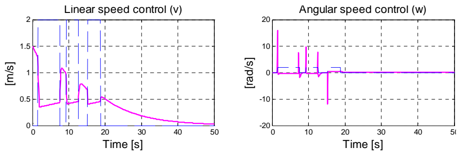
Fig. 7. Control without adaptive mechanism
