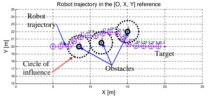
Fig. 5. Smooth robot trajectory obtained with the proposed control architecture
