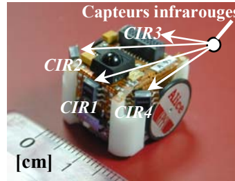
FIG. 4.2 – Mini-robot ALICE
