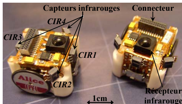
FIG. 8.4 – Mini-robots ALICE
